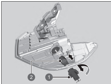
1 Socket 2 Bulb
